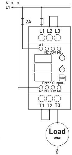
Connection Diagram (Mono-phase)
