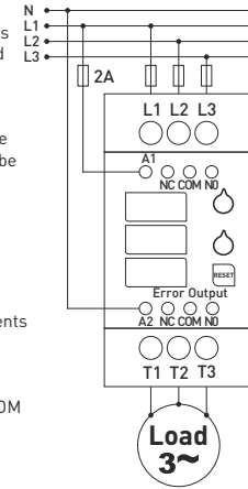
Connection Diagram (Three-phase)
